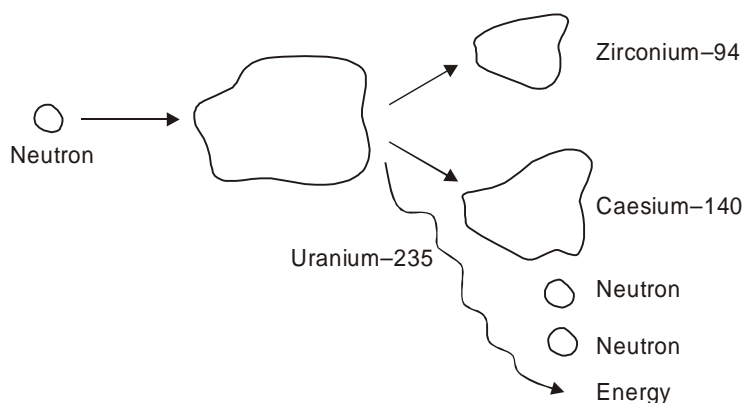
Fig. 7.3 Nuclear fission
